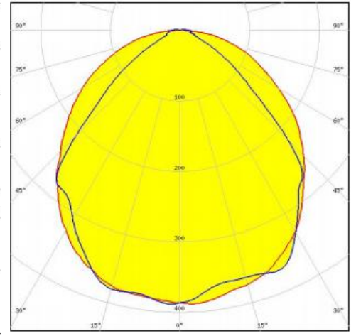
90° beam optimized for 2835led. Variant made from PC.
